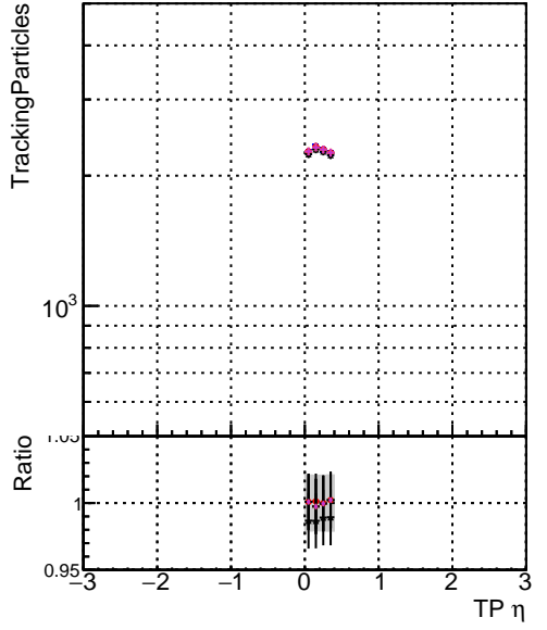
— DQM_original_step2_pt1to20_eta0p0to0p4 — DQM_angle_step2_pt1to20_eta0p0to0p4 — DQM_fast_step2_pt1to20_eta0p0to0p4 — DQM_mkFit_step2_pt1to20_eta0p0to0p4 — DQM_CPEpixel2_step2_pt1to20_eta0p0to0p4
