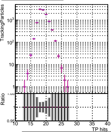
—●— DQM_original_step2_pt1to20_eta0p0to0p4 —●— DQM_angle_step2_pt1to20_eta0p0to0p4 —●— DQM_fast_step2_pt1to20_eta0p0to0p4 —●— DQM_mkFit_step2_pt1to20_eta0p0to0p4 —●— DQM_CPEpixel1_step2_pt1to20_eta0p0to0p4
