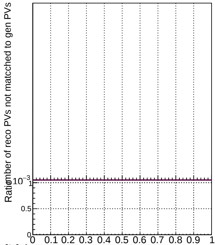
RecoPVAssoc2GenPVNotMatched_Purity
