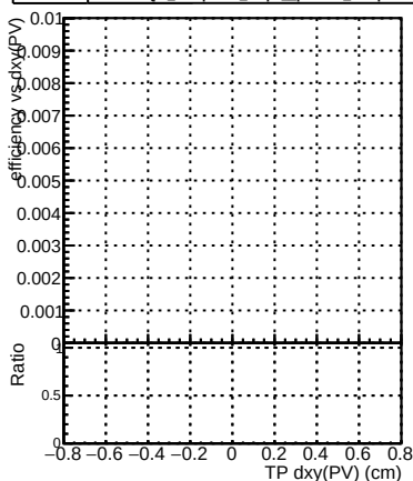
Efficienc DQM_mkFit_step2_pt1to20_eta0p0to0p4 DQM_CPEpixel1_step2_pt1to20_eta0p0to0p4
