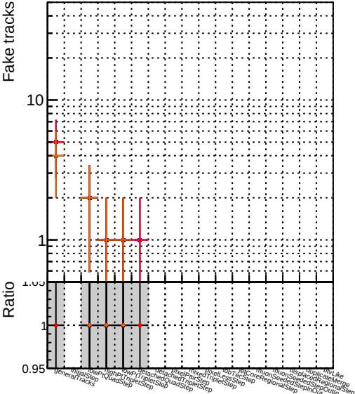
Number Legend Series —▲— DQM_testMkFitFit_step2_pt1to1000_eta2p6to4p0 —+— DQM_testMkFitFit_step2_pt1to1000_eta2p6to4p0_Rej10
