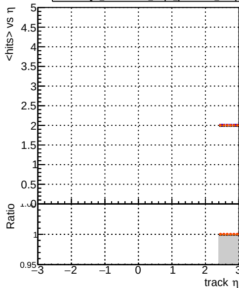
mean hits DQM_original4_step2_pt1to1000_eta2p6to4p0 DQM_testMkFit_step2_pt1to1000_eta2p6to4p0 DQM_testMkFitFit_step2_pt1to1000_eta2p6to4p0 DQM_testMkFitFit_step2_pt1to1000_eta2p6to4p0_Rej10
