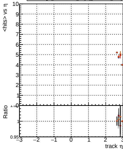
mean hits vs \eta DQM_original4_step2_pt1to1000_eta2p6to4p0 DQM_testMkFit_step2_pt1to1000_eta2p6to4p0 DQM_testMkFit_step2_pt1to1000_eta2p6to4p0 DQM_testMkFit_step2_pt1to1000_eta2p6to4p0_Rej10
