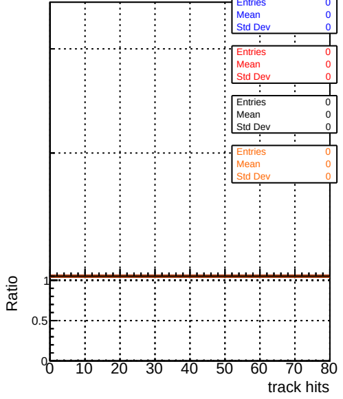
mean hit — DQM_original4_step2_pt1to1000_eta2p6to4p0 — DQM_testMkFit_step2_pt1to1000_eta2p6to4p0 — DQM_testMkFitFit_step2_pt1to1000_eta2p6to4p0 — DQM_testMkFitFit_step2_pt1to1000_eta2p6to4p0_Rej10
