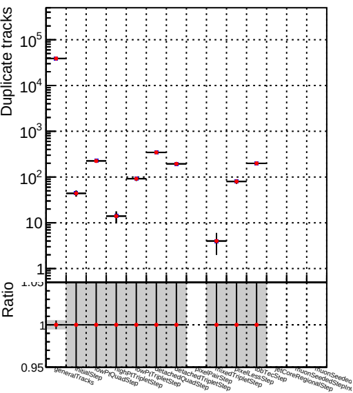
../CMSSW_13_2_X_2023-05-08-2300/src/DQM_TT_mkFit-DQM_new132
