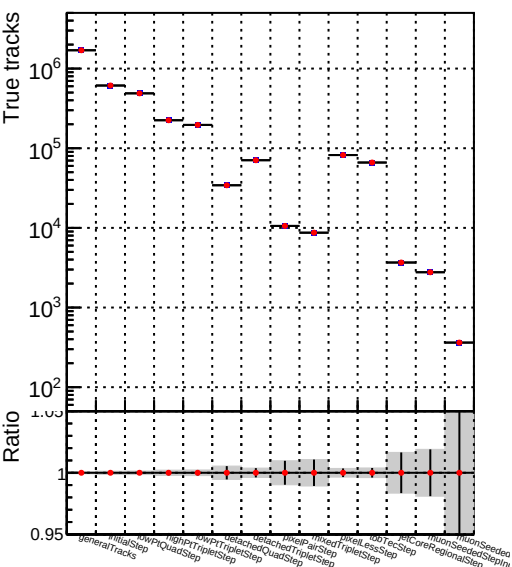
../CMSSW_13_2_X_2023-05-08-2300/src/DQM_TT_mkFit-DQM_new132
