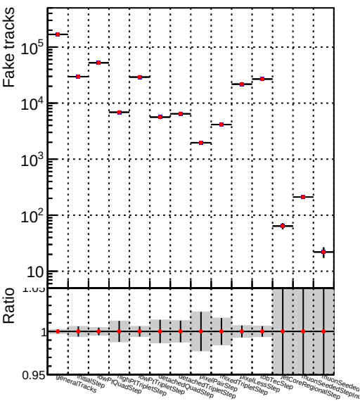
Numbe —●— DQM_TT_mkFit-DQM_newfastPlus132
