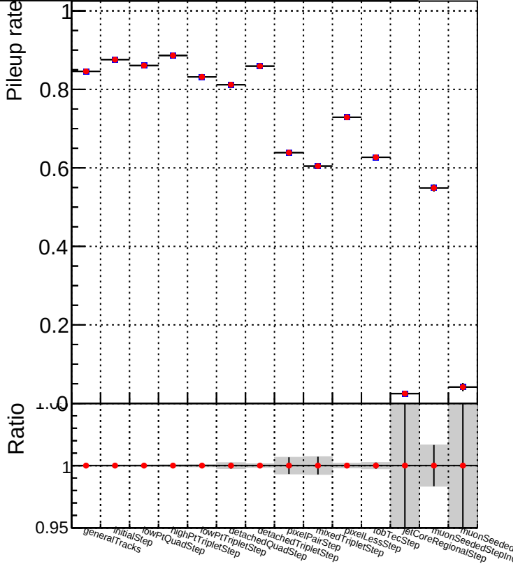
..../CMSSW_13_2_X_2023-05-08-2300/src/DQM_TT_mkFit-DQM_new132
