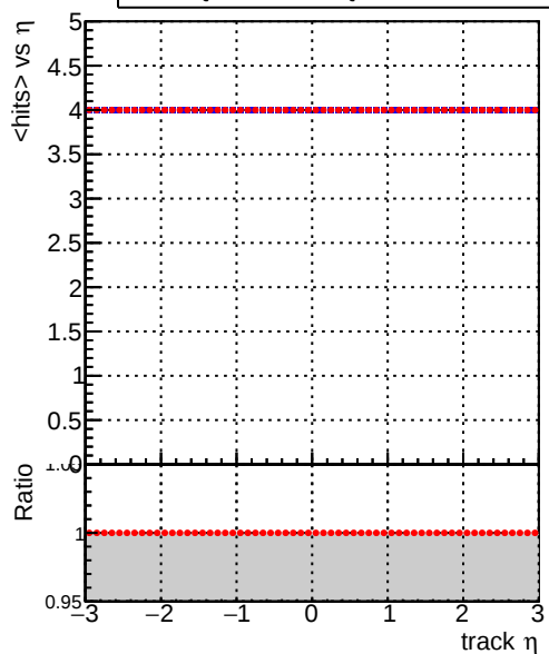
mean hits ././CMSSW_13_2_X_2023-05-08-2300/src/DQM_TT_mkFit-DQM_new132 DQM_TT_mkFit-DQM_newfastPlus132
