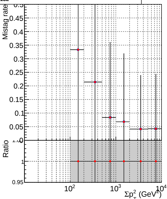
..../CMSSW_13_2_X_2023-05-08-2300/src/DQM_TT_mkFit-DQM_new132 DQM_TT_mkFit-DQM_newfastPlus132
