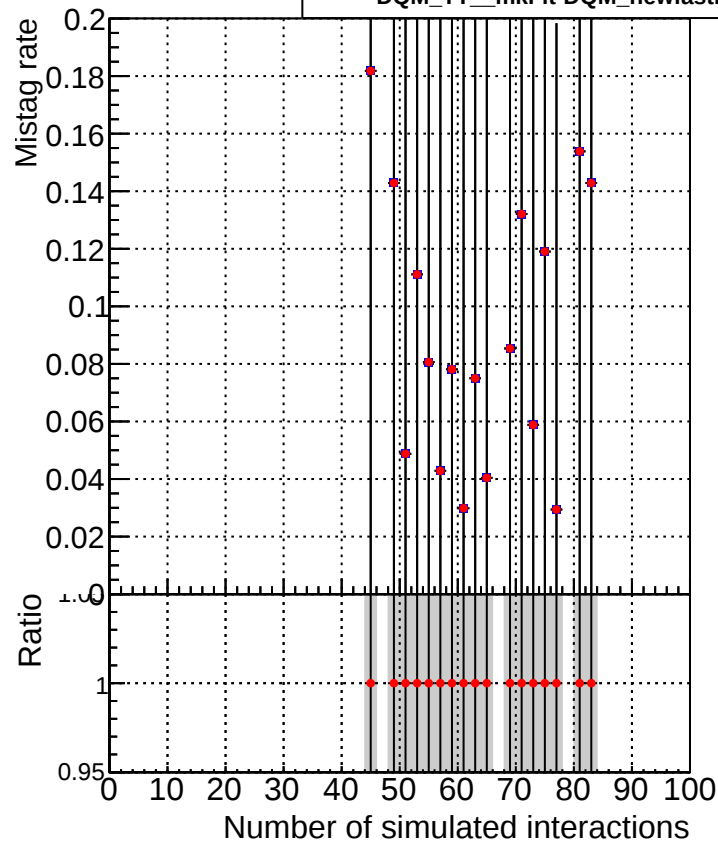
..../CMSSW_13_2_X_2023-05-08-2300/src/DQM_TT_mkFit-DQM_new132 DQM_TT_mkFit-DQM_newfastPlus132
