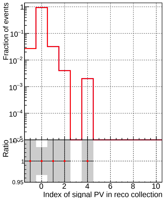
..../CMSSW_13_2_X_2023-05-08-2300/src/DQM_TT_mkFit-DQM_new132 DQM_TT_mkFit-DQM_newfastPlus132
