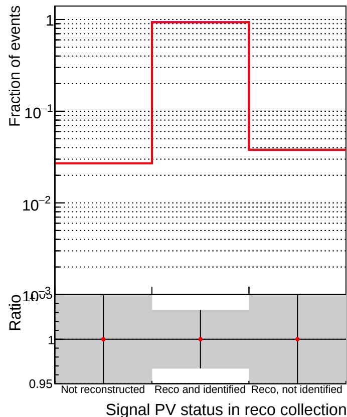
..../CMSSW_13_2_X_2023-05-08-2300/src/DQM_TT_mkFit-DQM_new132 DQM_TT_mkFit-DQM_newfastPlus132
