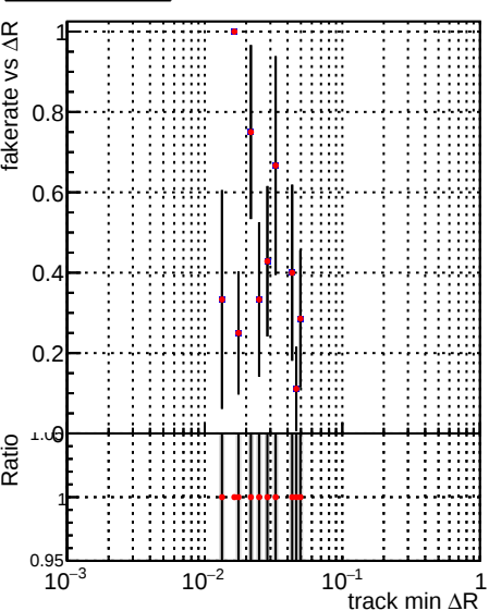
█ ● ../CMSSW_13_2_X_2023-05-08-2300/src/DQM_TT_mkFit-DQM_new132 █ ● DQM_TT_mkFit-DQM_newfastPlus132
