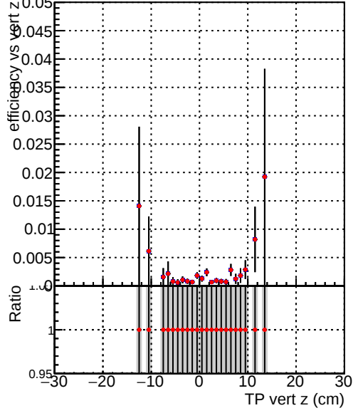
Efficiency vs. TP vert z - - ././CMSSW_13_2_X_2023-05-08-2300/src/DQM_TT_mkFit-DQM_new132 - - DQM_TT_mkFit-DQM_newfastPlus132
