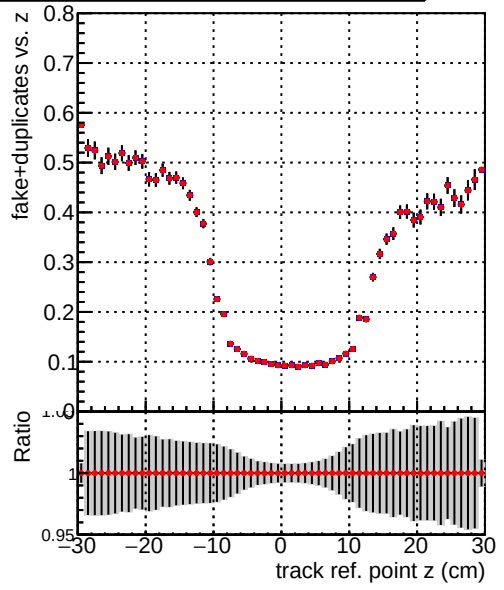
Efficiency vs. TP vert z (cm) (Left) and fake+duplicates vs. track ref. point z (cm) (Right)
