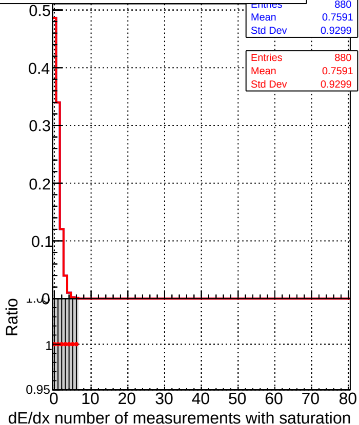
Legend: - Grey histogram: ../CMSSW_13_2_X_2023-05-08-2300/src/DQM_TT_mkFit-DQM_new132 - Red line with dots: DQM_TT_mkFit-DQM_newfastPlus132
