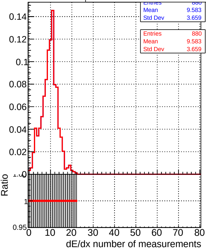
Legend: - Grey histogram: ../CMSSW_13_2_X_2023-05-08-2300/src/DQM_TT_mkFit-DQM_new132 - Red line with dots: DQM_TT_mkFit-DQM_newfastPlus132
