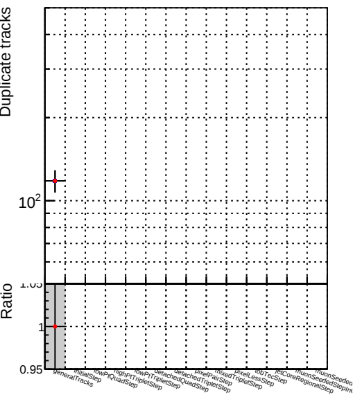
Number —●— DQM_TT_mkFit-DQM_newfastPlus132
