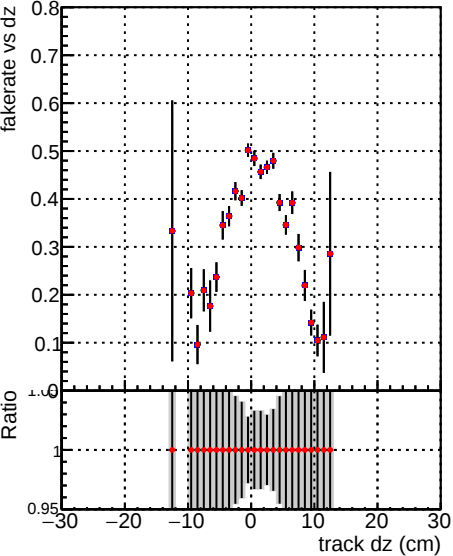
Fake rate vs dz Legend: - Blue dots: /..../CMSSW_13_2_X_2023-05-08-2300/src/DQM_TT_mkFit-DQM_new132 - Red dots: DQM_TT_mkFit-DQM_newfastPlus132
