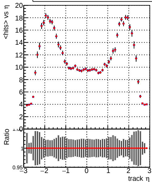
mean hits vs \eta ./../CMSSW_13_2_X_2023-05-08-2300/src/DQM_TT_mkFit-DQM_new132 DQM_TT_mkFit-DQM_newfastPlus132
