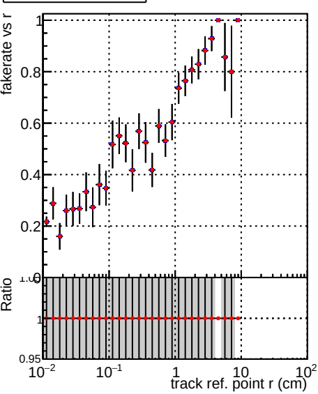
Legend: - \bullet ../CMSSW_13_2_X_2023-05-08-2300/src/DQM_TT_mkFit-DQM_new132 - \bullet DQM_TT_mkFit-DQM_newfastPlus132
