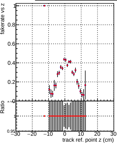
Legend: - \bullet ../CMSSW_13_2_X_2023-05-08-2300/src/DQM_TT_mkFit-DQM_new132 - \bullet DQM_TT_mkFit-DQM_newfastPlus132
