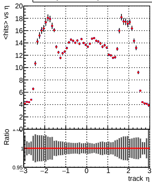
mean hit ./.CMSSW_13_2_X_2023-05-08-2300/src/DQM_TT_mkFit-DQM_new132 DQM_TT_mkFit-DQM_newfastPlus132
