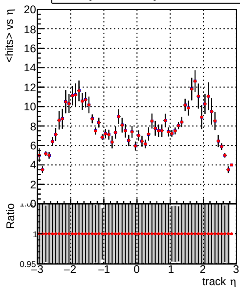
mean hits vs \eta Legend: - ./././CMSSW_13_2\_X\_2023-05-08-2300/src/DQM\_TT\_mkFit-DQM\_new132 (blue line) - DQM\_TT\_mkFit-DQM\_newfastPlus132 (red line)
