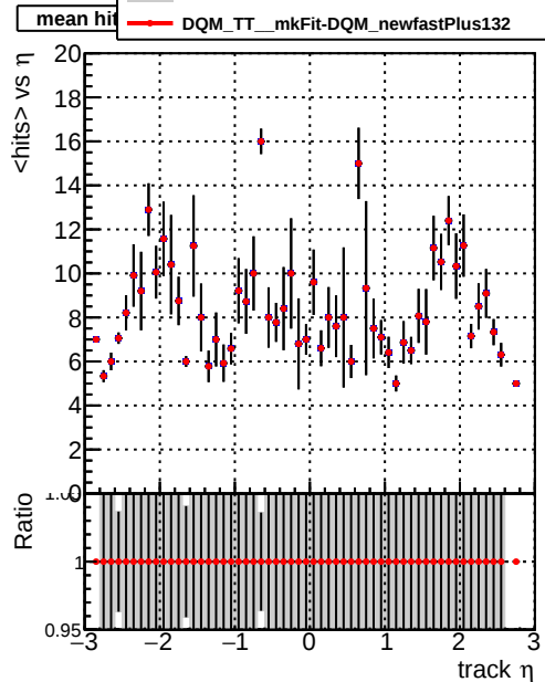
mean hits vs \eta
