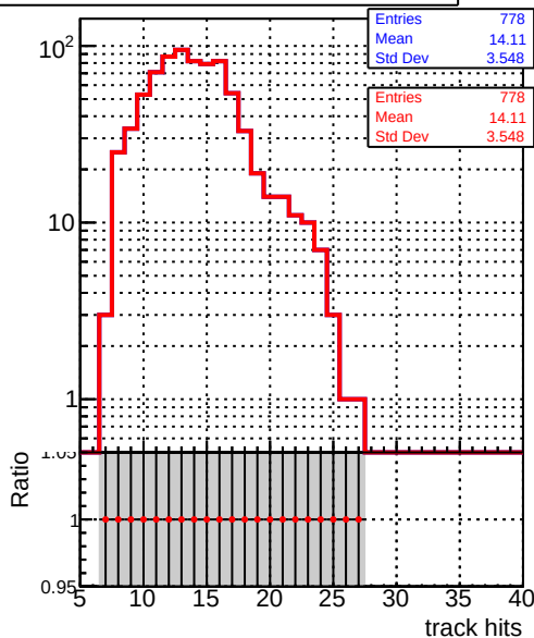
mean hit ./../CMSSW_13_2_X_2023-05-08-2300/src/DQM_TT_mkFit-DQM_new132 DQM_TT_mkFit-DQM_newfastPlus132
