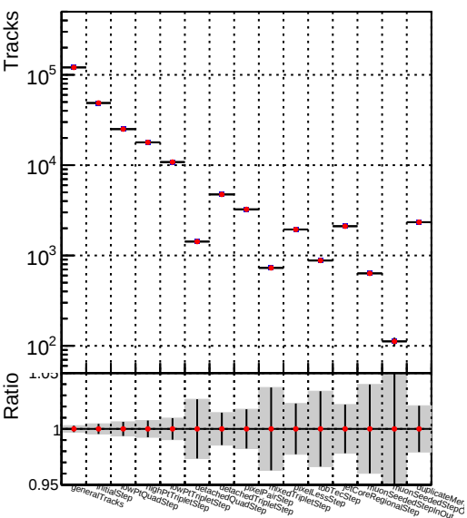
../CMSSW_13_2_X_2023-05-08-2300/src/DQM_TT_mkFit-DQM_new132
