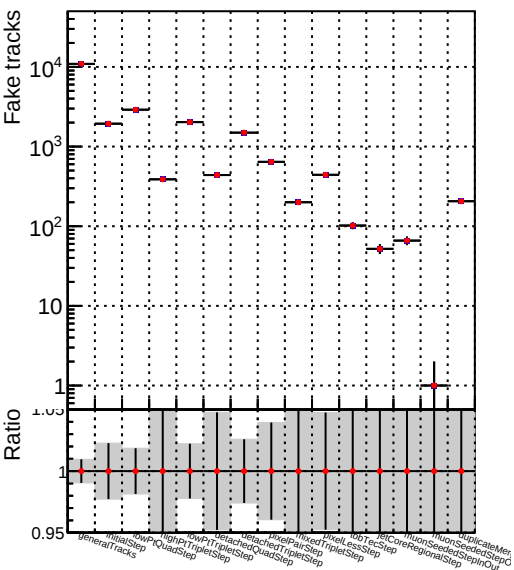
Number —●— DQM_TT_mkFit-DQM_newfastPlus132
