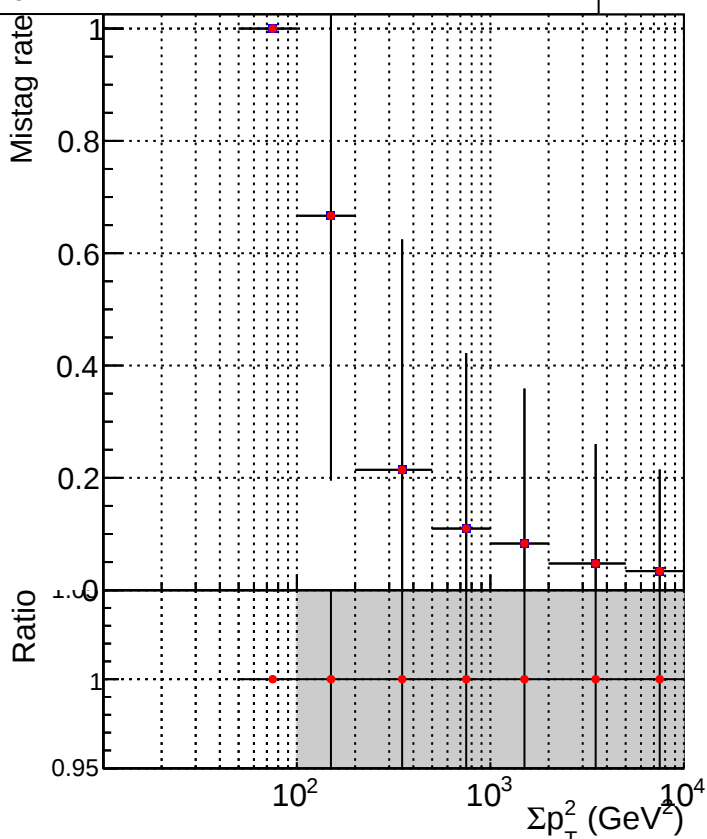
..../CMSSW_13_2_X_2023-05-08-2300/src/DQM_TT_mkFit-DQM_new132 DQM_TT_mkFit-DQM_newfastPlus132
