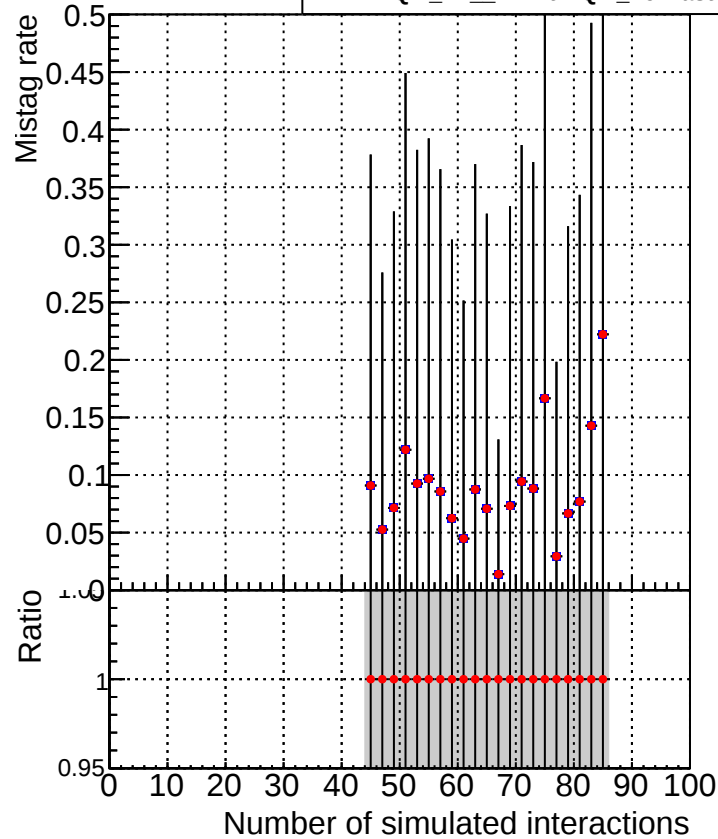
..../CMSSW_13_2_X_2023-05-08-2300/src/DQM_TT_mkFit-DQM_new132 DQM_TT_mkFit-DQM_newfastPlus132
