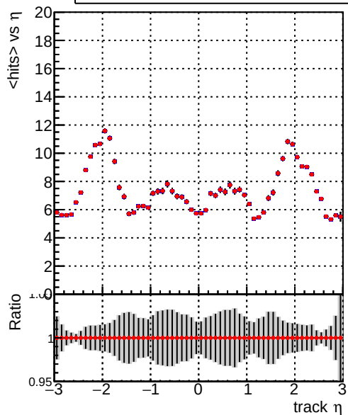
./../CMSSW_13_2_X_2023-05-08-2300/src/DQM_TT_mkFit-DQM_new132 mean hits DQM_TT_mkFit-DQM_newfastPlus132
