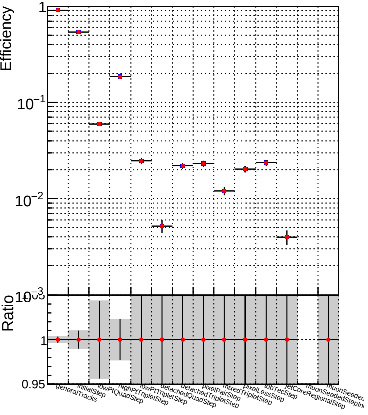
Legend: - ../CMSSW_13_2_X_2023-05-08-2300/src/DQM_TT_mkFit-DQM_new132 - DQM_TT_mkFit-DQM_newfastPlus132
