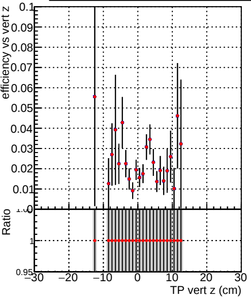
Efficiency vs vertpos Legend: \bullet ./../CMSSW_13_2_X_2023-05-08-2300/src/DQM_TT_mkFit-DQM_new132 \bullet DQM_TT_mkFit-DQM_newfastPlus132
