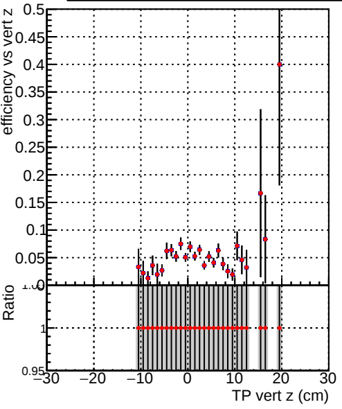
Efficiency vs vert z Legend: - ./../CMSSW_13_2_X_2023-05-08-2300/src/DQM_TT_mkFit-DQM_new132 (blue line with dots) - DQM_TT_mkFit-DQM_newfastPlus132 (red line with dots)
