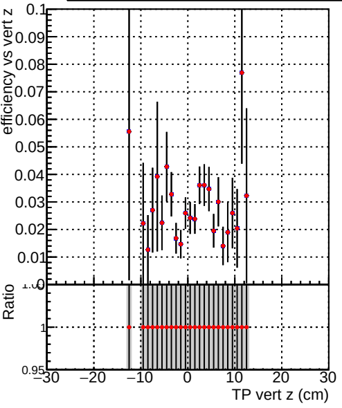
Efficiency vs vertpos Legend: - ./../CMSSW_13_2_X_2023-05-08-2300/src/DQM_TT_mkFit-DQM_new132 (Blue line with dots) - DQM_TT_mkFit-DQM_newfastPlus132 (Red line with dots)
