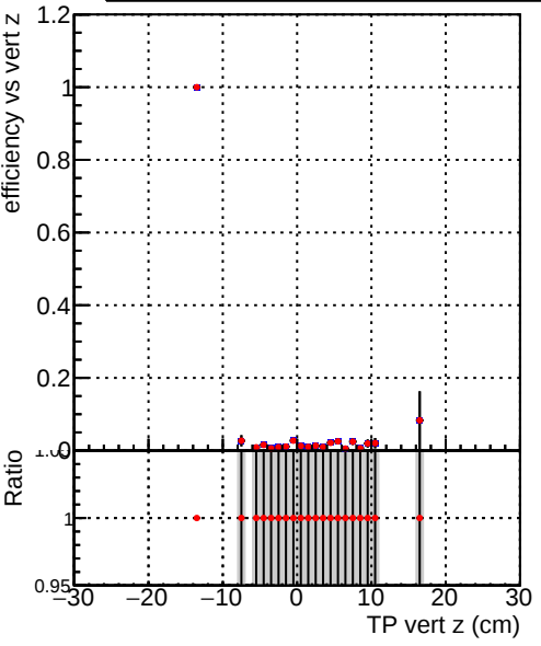
Efficiency vs vert z Legend: ./../CMSSW_13_2_X_2023-05-08-2300/src/DQM_TT_mkFit-DQM_new132 DQM_TT_mkFit-DQM_newfastPlus132
