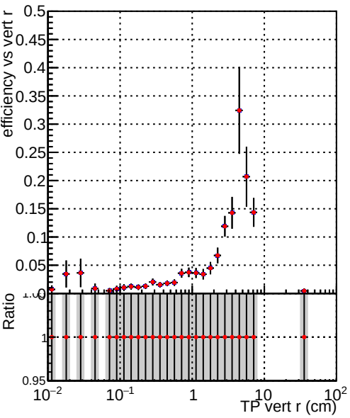
Efficiency vs TP vert r (cm) ././CMSSW_13_2_X_2023-05-08-2300/src/DQM_TT_mkFit-DQM_new132 DQM_TT_mkFit-DQM_newfastPlus132
