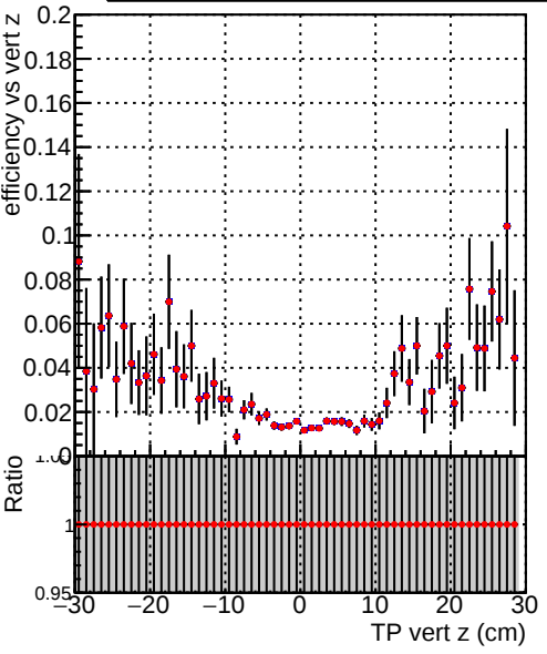
Efficiency vs TP vert z (cm) Legend: - ././CMSSW_13_2_X_2023-05-08-2300/src/DQM_TT_mkFit-DQM_new132 (Blue line with markers) - DQM_TT_mkFit-DQM_newfast132 (Red line with markers)
