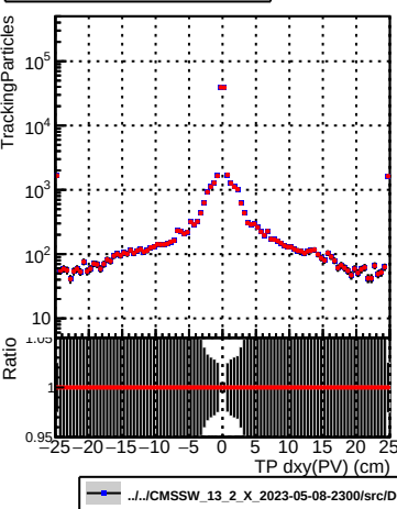
N of sim DQM_TT_mkFit-DQM_newfast132
