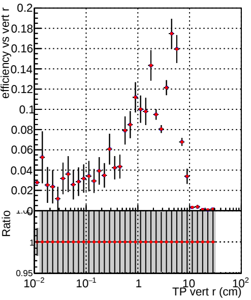
Efficiency vs TP vert r (cm) Legend: ././CMSSW_13_2_X_2023-05-08-2300/src/DQM_TT_mkFit-DQM_new132 DQM_TT_mkFit-DQM_newfast132
