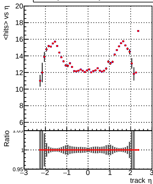
mean hits vs \eta Legend: ./././CMSSW_13_2_X_2023-05-08-2300/src/DQM\_TT\_mkFit-DQM\_new132 (blue line), DQM\_TT\_mkFit-DQM\_newfast132 (red line)
