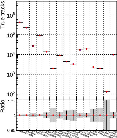
./../CMSSW_13_2_X_2023-05-08-2300/src/DQM_TT_mkFit-DQM_new132
