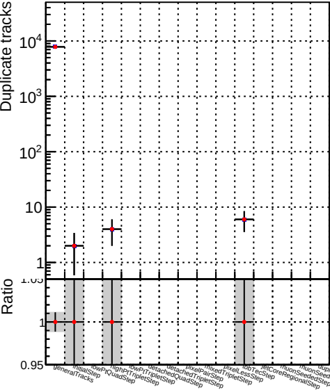
./../CMSSW_13_2_X_2023-05-08-2300/src/DQM_TT_mkFit-DQM_new132
