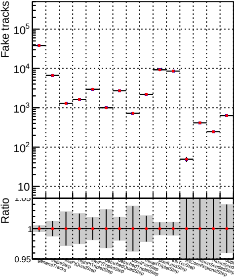
Number —●— DQM_TT_mkFit-DQM_newfast132
