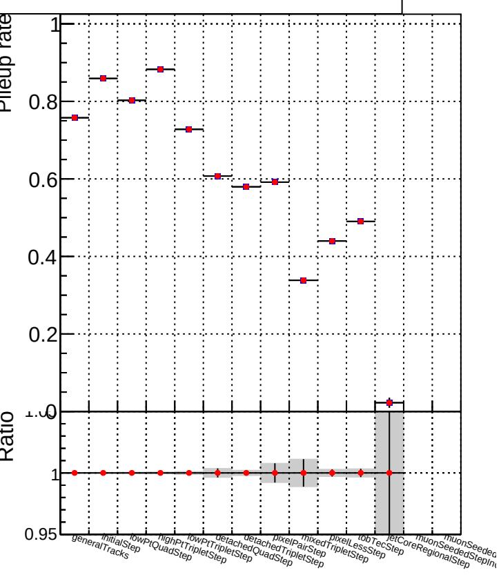
../CMSSW_13_2_X_2023-05-08-2300/src/DQM_TT_mkFit-DQM_new132
