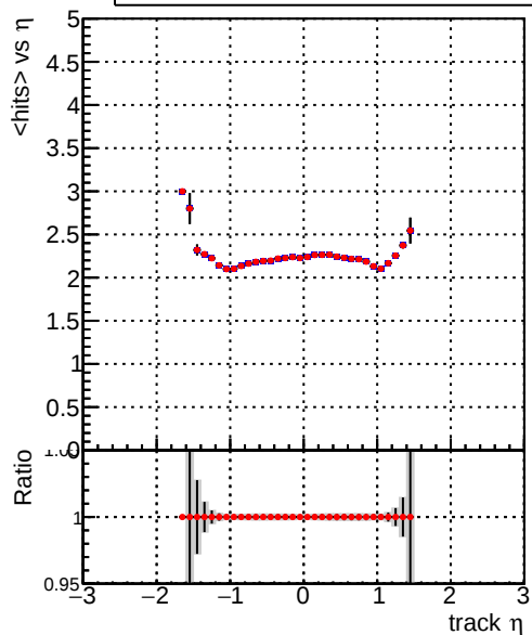
mean hits vs \eta ././CMSSW_13_2_X_2023-05-08-2300/src/DQM_TT_mkFit-DQM_new132 DQM_TT_mkFit-DQM_newfast132
