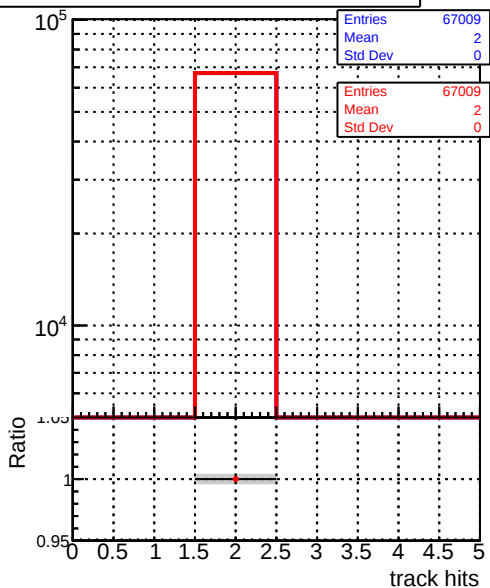
mean hit ..../CMSSW_13_2_X_2023-05-08-2300/src/DQM_TT_mkFit-DQM_new132 DQM_TT_mkFit-DQM_newfast132
