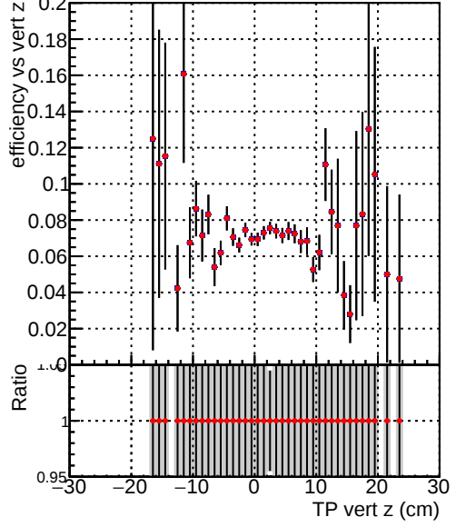
Efficiency vs. TP vert z Legend: - ./././CMSSW_13_2\_X\_2023-05-08-2300/src/DQM\_TT\_mkFit-DQM\_new132 (blue line) - DQM\_TT\_mkFit-DQM\_newfast132 (red line)
