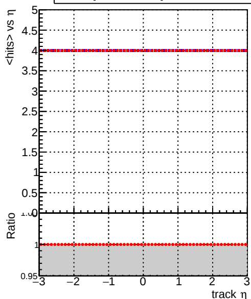
mean hits ./../CMSSW_13_2_X_2023-05-08-2300/src/DQM_TT_mkFit-DQM_new132 DQM_TT_mkFit-DQM_newfast132
