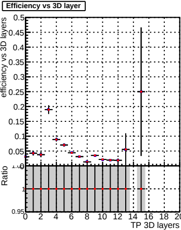
Efficiency vs 3D layer
