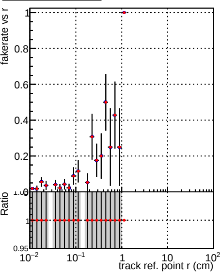
Fake rate vs v ..../CMSSW_13_2_X_2023-05-08-2300/src/DQM_TT_mkFit-DQM_new132 DQM_TT_mkFit-DQM_newfast132
