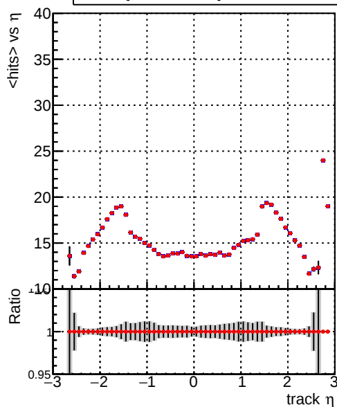
./../CMSSW_13_2_X_2023-05-08-2300/src/DQM_TT_mkFit-DQM_new132 mean hits vs \eta DQM_TT_mkFit-DQM_newfast132
