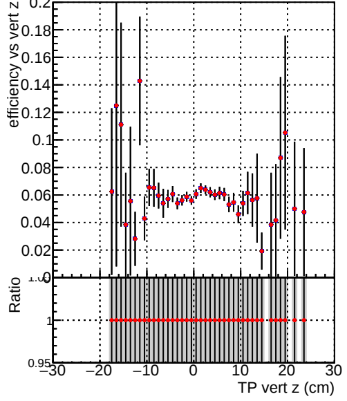
Efficiency vs. TP vert z (cm) vs. Sim. PV z (cm) Legend: ./././CMSSW_13_2\_X\_2023-05-08-2300/src/DQM\_TT\_mkFit-DQM\_new132 DQM\_TT\_mkFit-DQM\_newfast132
