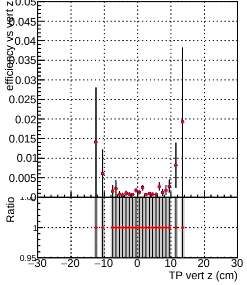
Efficiency vs. sim PV z Legend: - ./././CMSSW_13\_2\_X\_2023-05-08-2300/src/DQM\_TT\_mkFit-DQM\_new132 (grey bars) - DQM\_TT\_mkFit-DQM\_newfast132 (red dots)
