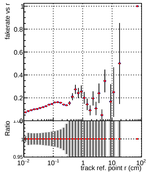
Legend: - \dots ../CMSSW_13_2_X_2023-05-08-2300/src/DQM_TT_mkFit-DQM_new132 - \dots DQM_TT_mkFit-DQM_newfast132
